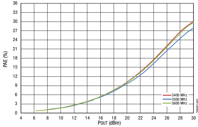
Figure 3. PAE vs POUT Across Frequency @ 5 V 25 °C
