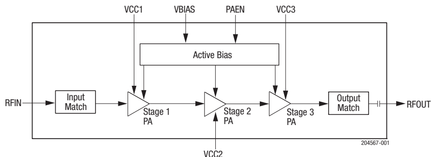
Figure 1. SKY66313-11 Block Diagram
