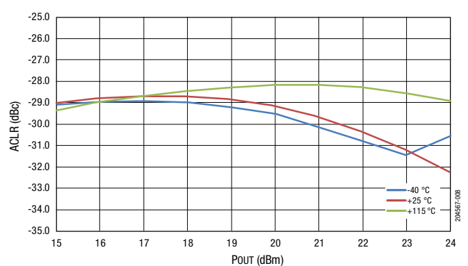
Figure 8. ACLR-5C vs POUT Across Temperature @ 3500 MHz, 5 V
