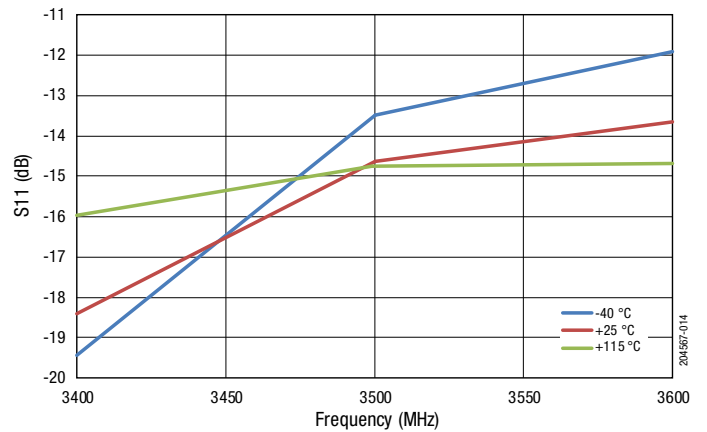
Figure 14. S11 vs Frequency Across Temperature
