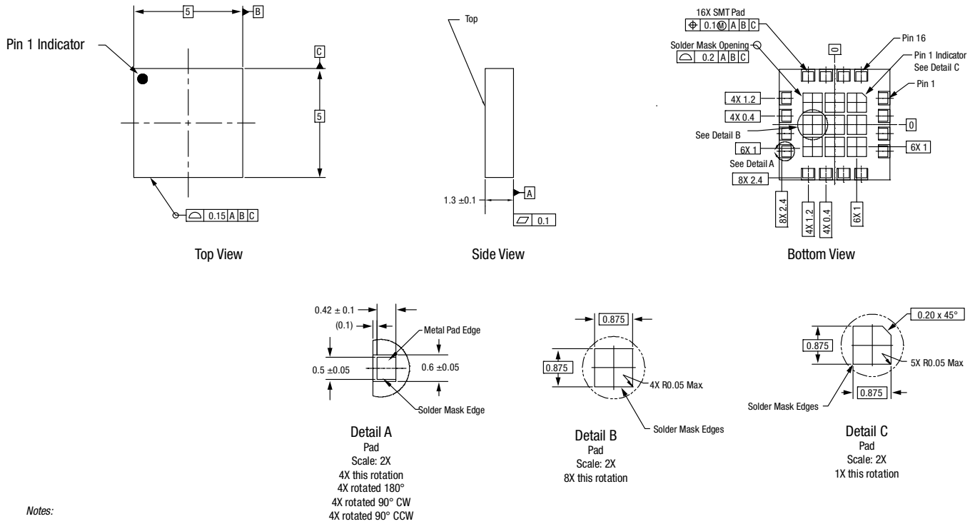
Figure 30. SKY66313-11 Package Dimensions
