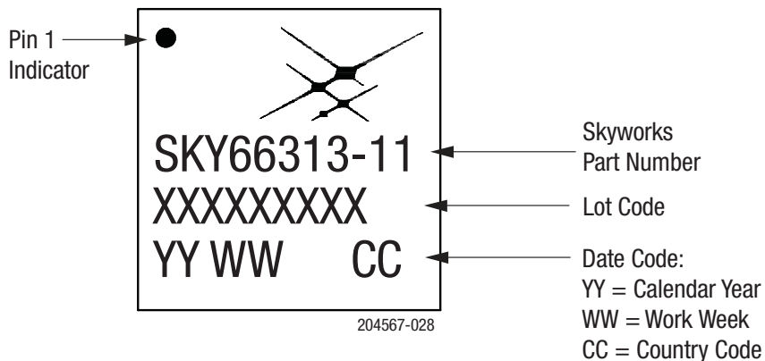
Figure 28. SKY66313-11 Typical Part Marking
