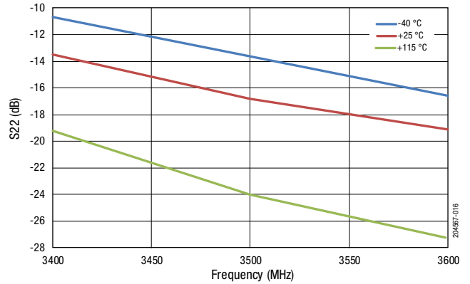
Figure 16. S22 vs Frequency Across Temperature
