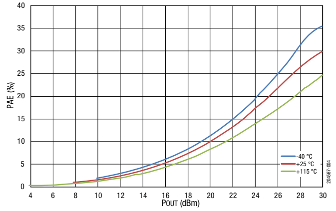
Figure 4. PAE vs POUT Across Temperature @ 3500 MHz, 5 V
