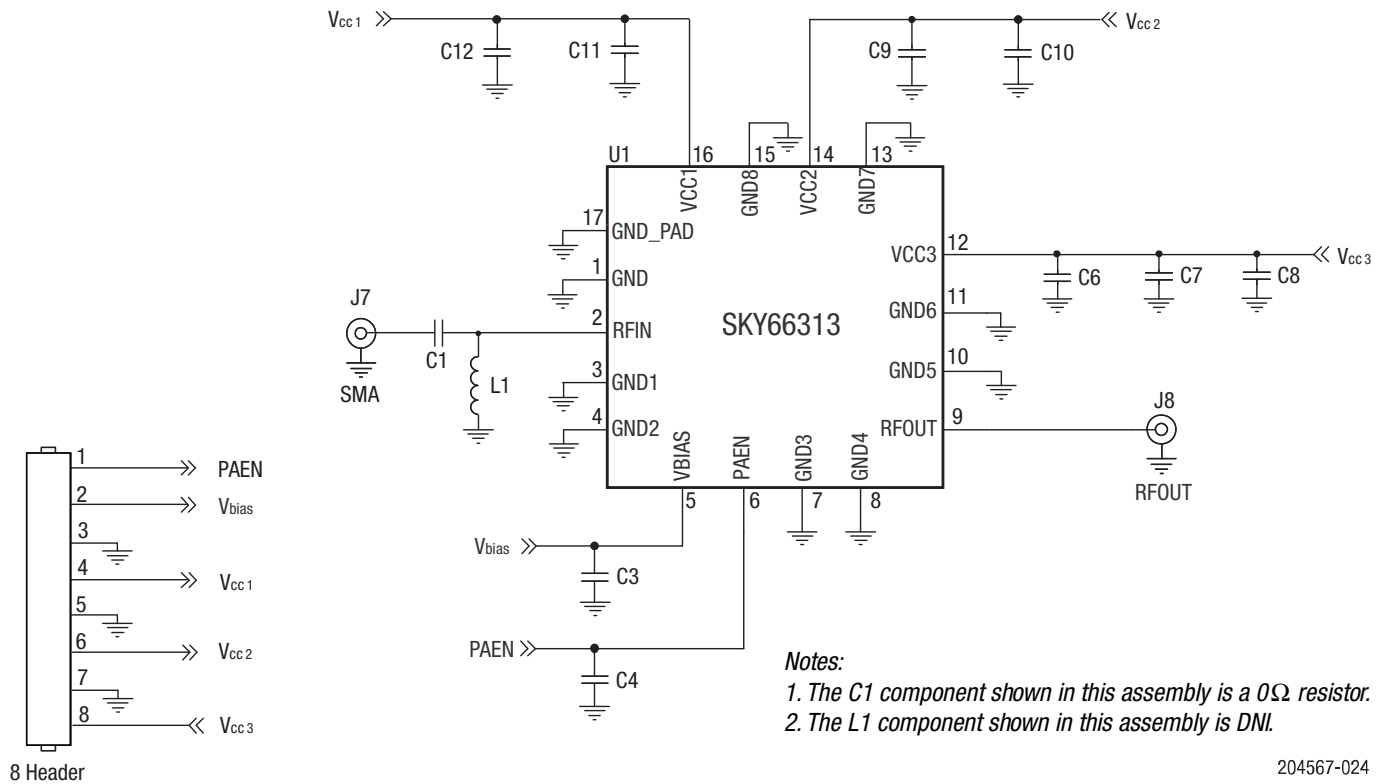
Figure 24. SKY66313-11 Application Schematic
