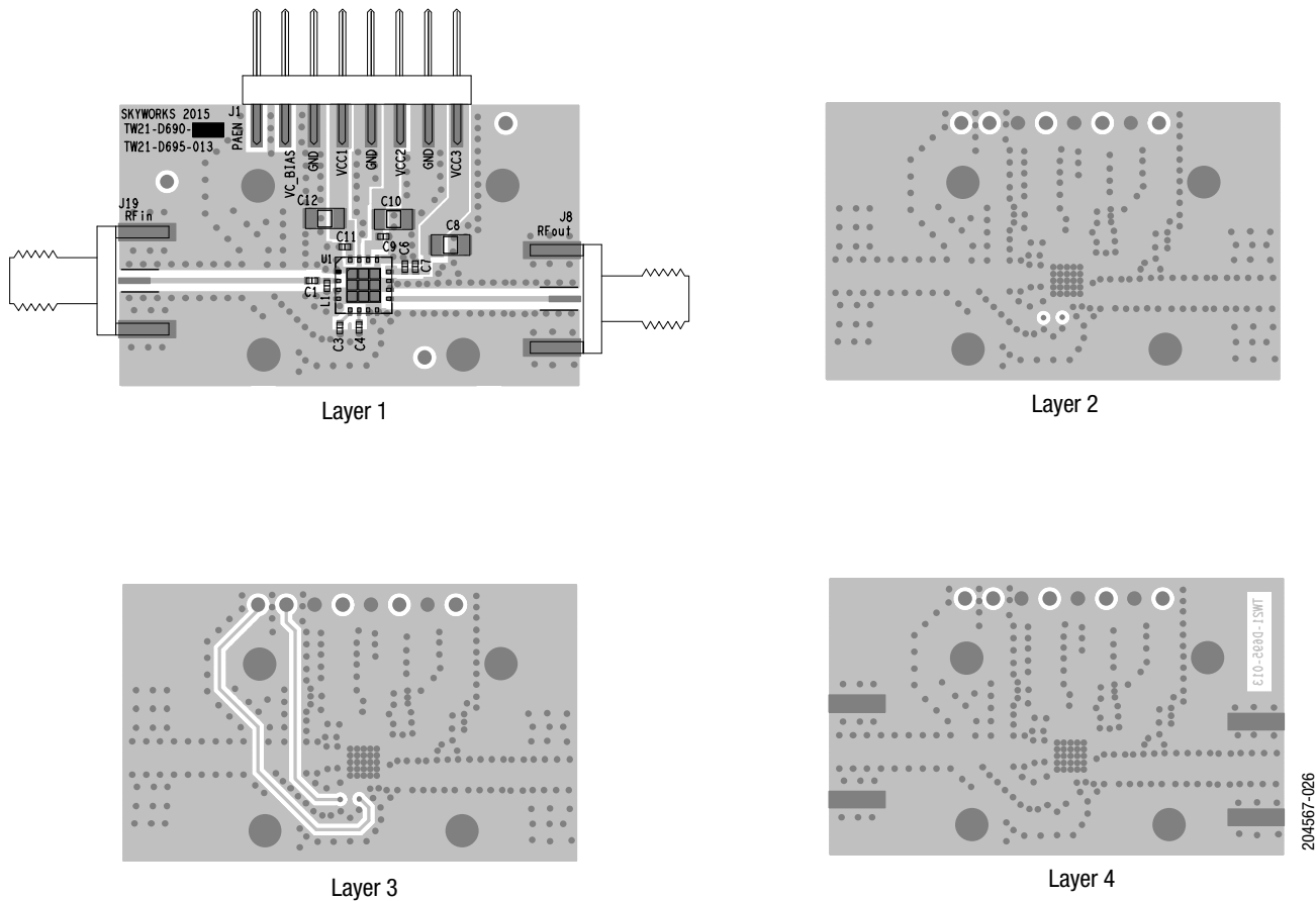
Figure 26. Board Layer Detail
