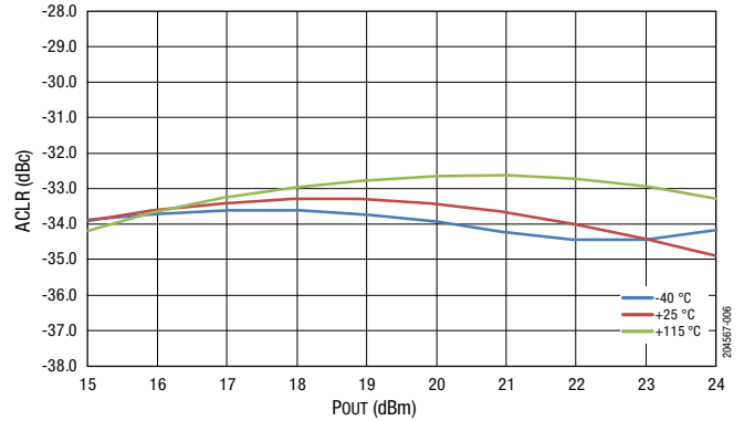
Figure 6. ACLR-1C vs POUT Across Temperature @ 3500 MHz, 5 V
