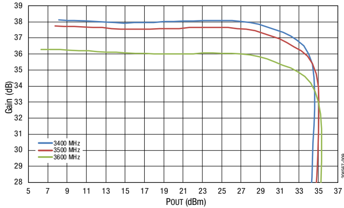
Figure 9. Gain vs POUT Across Frequency @ 5 V 25 °C
